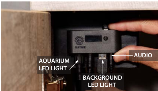
12 Connect LED light to controller (insert then screw tighten), slide-in background light USB plug, then connect small audio speaker plug.
